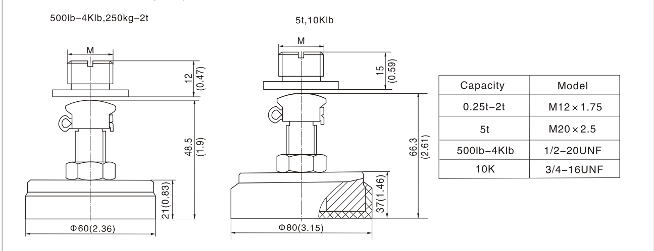
Stainless steel, assembled with: BM8H,H8H
