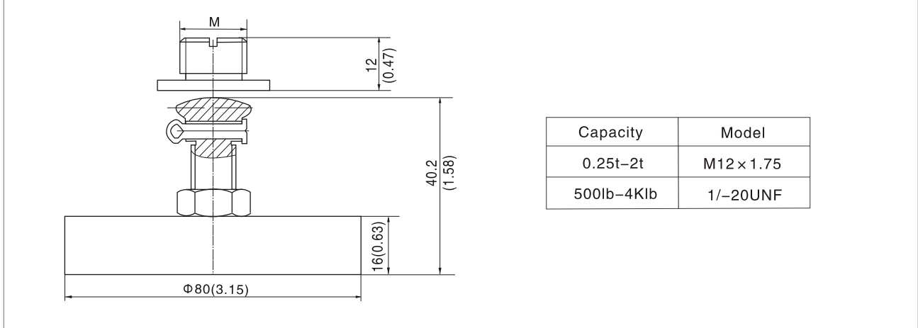
Stainless steel, assembled with: BM8H,H8H
