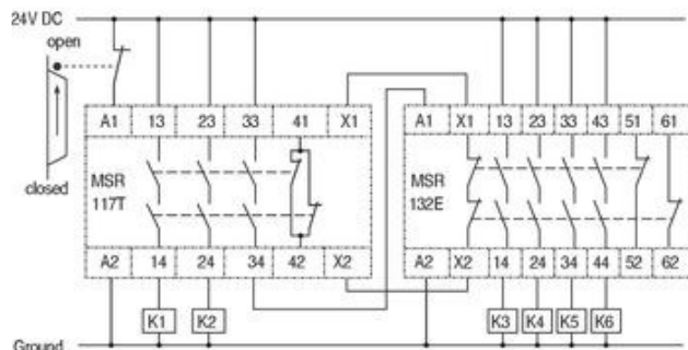
Single Channel Gate Interlock, Automatic Reset, Single Channel Output Expansion
