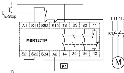
Single Channel E-Stop, Automatic Reset, No Output Monitoring
